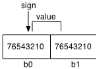
Fig. 5C-23. Signed bit string
