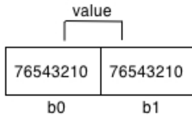
Fig. 5C-24. Unsigned bit string
