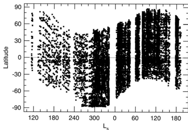
Figure 1. The seasonal ( L_s ) and latitudinal distribution of CRISM retrievals. Gaps near the winter poles are from the requirement that solar incidence angle be no larger than 80^\circ and that the ground be free of surface ice. Vertical gaps were caused by solar conjunction and recovery from spacecraft anomalies.
