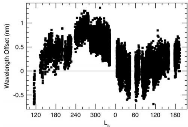
Figure 7. The retrieved wavelength calibration offset as a function of season ( L_s ). The offset is small compared with the spectral resolution ( \sim 15 nm), but including it improves the retrievals.
