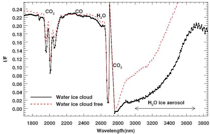
Figure 2. An example of a portion of the near-nadir Compact Reconnaissance Imaging Spectrometer for Mars spectrum (solid black) from observation EPF0000BD4B taken in July 2008 at L_s = 105 (M Y 29), and centered at 21.56N latitude, 16.15W longitude. The absorption bands from \text{CO}_2 , \text{H}_2\text{O} , and CO are indicated, and the large water ice aerosol feature is detected in the 3,000–3,700 nm range. The reflectances at 3,380 and 3,520 nm are used to calculate the water ice opacity index. In comparison, the normalized dashed red spectrum corresponds to cloud-free observation EPF000054C1 taken at L_s = 217 (M Y 28) and centered at 21.46S latitude and 52.71W longitude.
