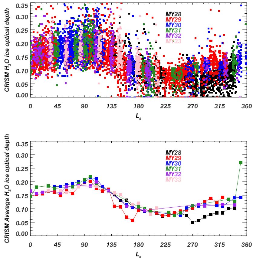
Figure 10. (top) Seasonal variation of the zonally averaged Compact Reconnaissance Imaging Spectrometer for Mars water ice aerosol optical depth for 5+ Martian year in the latitude bin 10S to 30N. The latitudes are chosen to capture the behavior of the aphelion cloud belt. (bottom) Same as the top panel but with an averaging of the optical depth using a seasonal bin of 10 in L_s to identify possible interannual variabilities.
