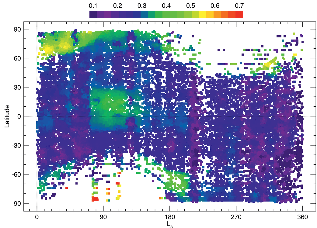
Figure 3. The seasonal dependence of the atmospheric water ice aerosol opacity index around 3.4 \mu\text{m} using the Compact Reconnaissance Imaging Spectrometer for Mars hyperspectral observations. The index is a metric of the aerosol band depth and is unitless, where a higher index indicates thicker/denser/more frequent water ice clouds. As observed, the annual cycle of water ice clouds with its distinctive aphelion cloud belt, north and south polar hoods is well depicted here.
