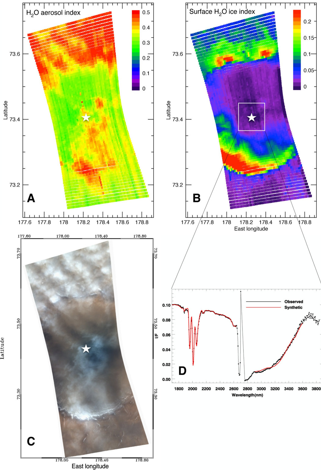
Figure 7. Panel (a) shows the retrieved ice aerosol opacity index (see Section 2.2) for observation HRL0000AA2A, taken on 28 April 2008 during later northern spring and centered at longitude 178.26E and latitude 73.41N. Panel (b) shows the surface ice index (see Section 3.3), and panel (c) shows the enhanced visible color image. The square in the middle of panel (b) indicates the central 100 \times 100 pixels from which the coadded spectrum used for the observation is extracted. Panel (d) shows the observed and fitted spectra of the observation in black and red, respectively.
