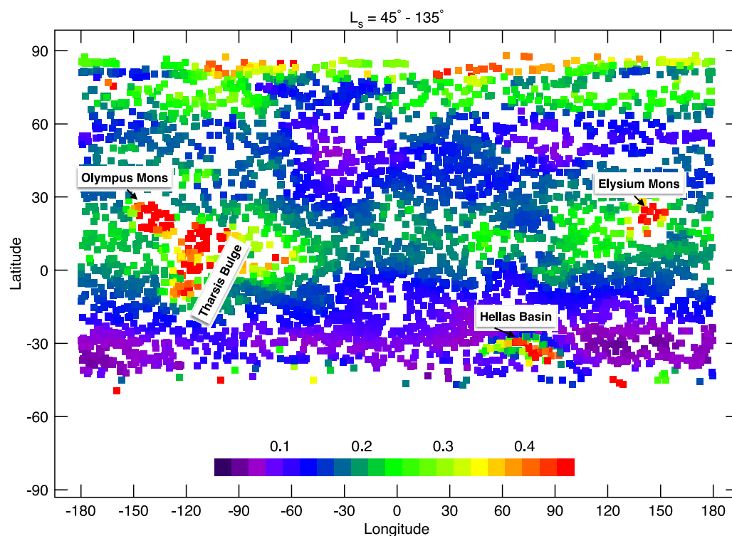
Figure 11. Retrieved Compact Reconnaissance Imaging Spectrometer for Mars water ice optical depth combined into one Martian year and averaged for the aphelion season between L_s = 45 and 135 to display the geographic enhancement in optical depth inside the aphelion cloud belt. The results are convolved using a boxcar kernel with a 20 \times 5 longitude – latitude size.
