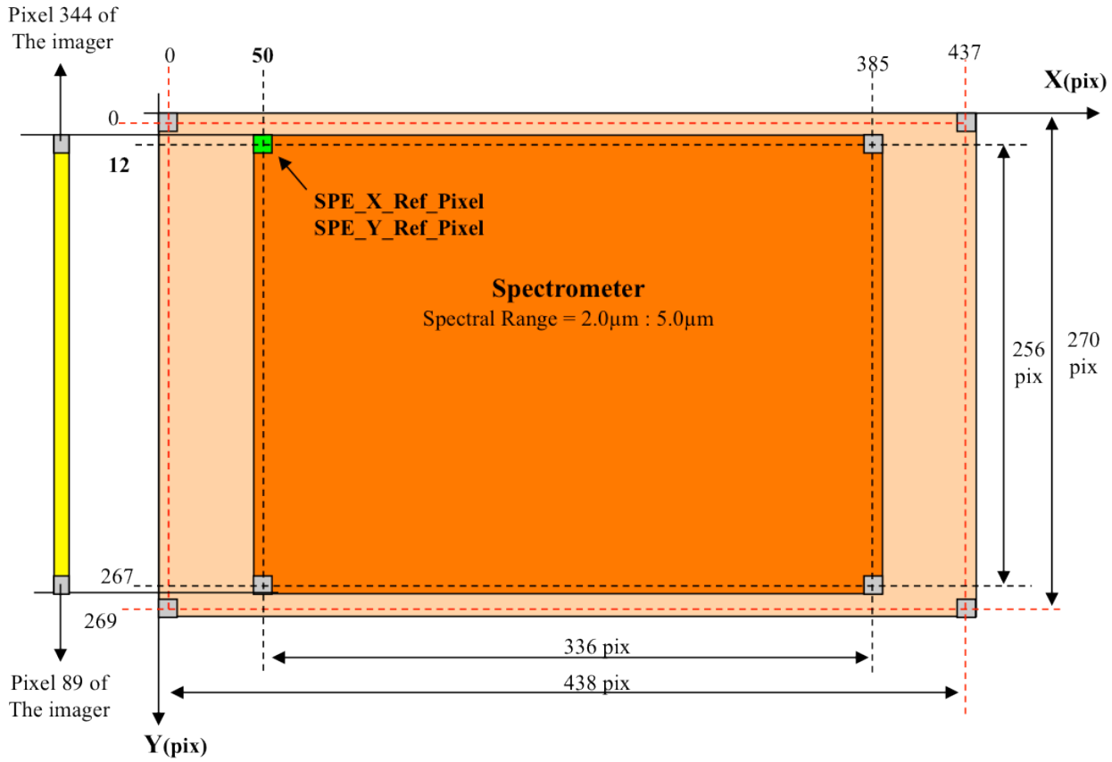
Figure 4: The Spectrometer focal plane
