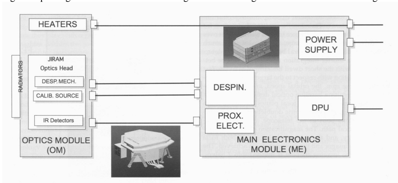
Figure 5: General block diagram of JIRAM. The electronic box contains the proximity and main electronics. Calib. Source, calibration source; Desp. Mech, de-spinning mechanism; DPU, Digital Processing Unit; Prox. Elect, proximity electronics.
