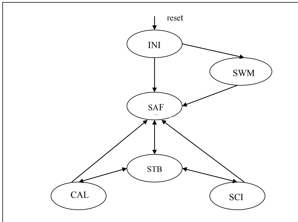
Figure 6: JIRAM FSW modes
