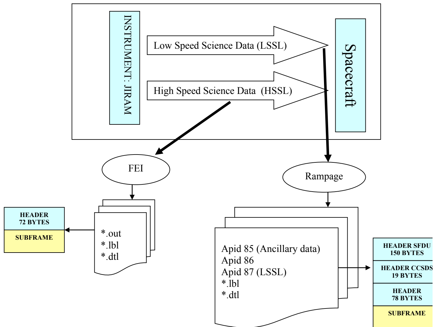
Figure 14: JIRAM Raw Science Data Product Pack
